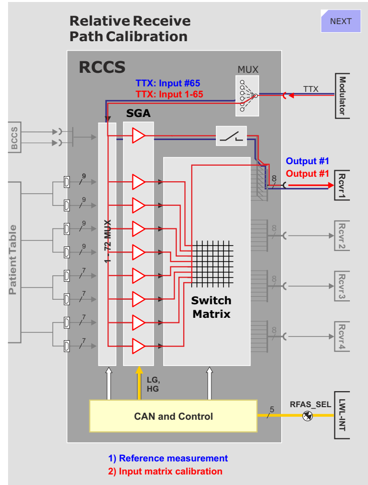
Figure 233 Receive Path Calibration: Steps 1 and 2
