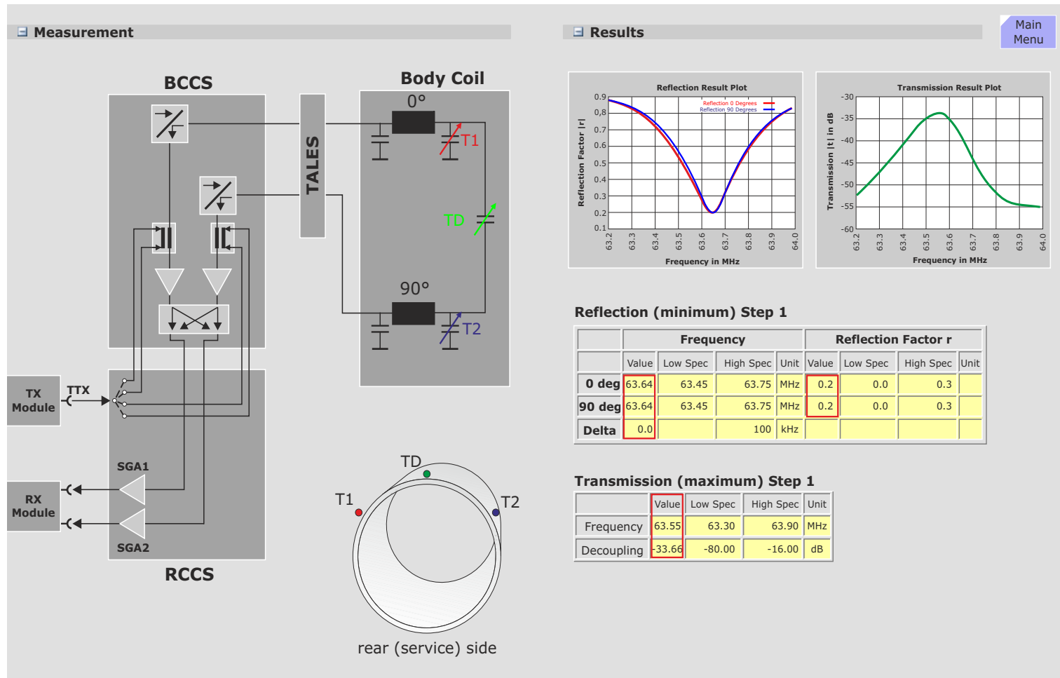
Figure 212 Body Coil Tuning and Decoupling Adjustments
