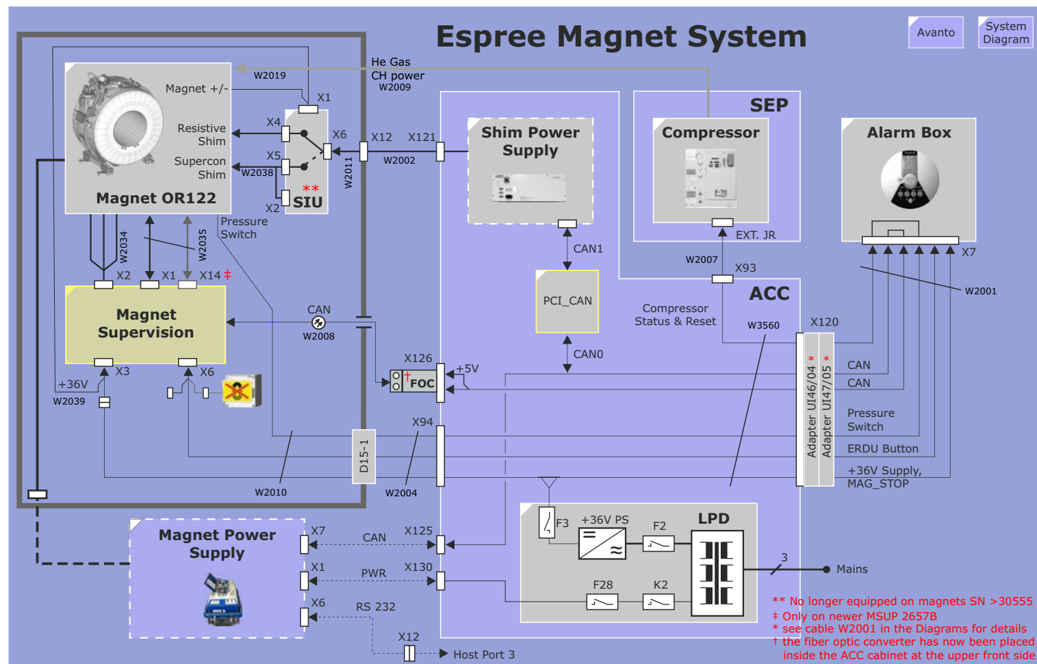
Figure 160 Espree Magnet System
