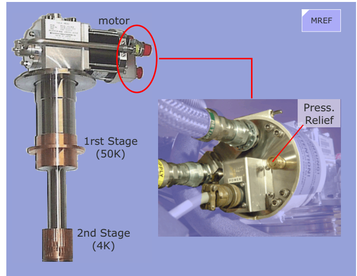
Figure 187 Cold Head (removed from Magnet)
