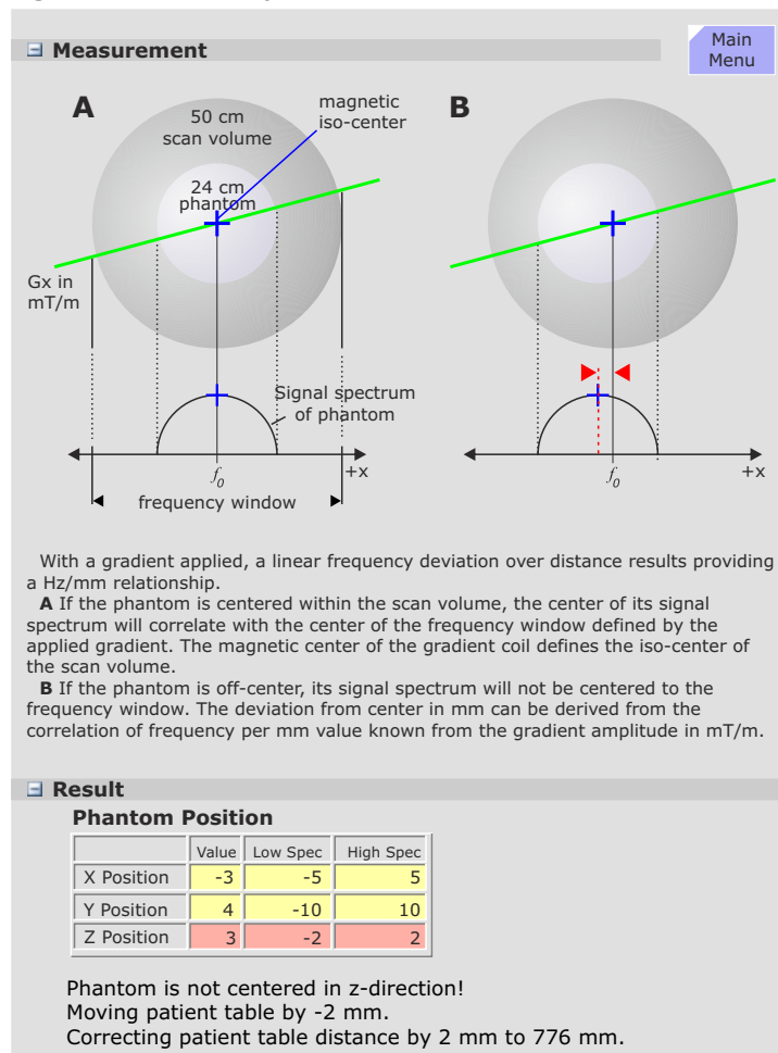
Figure 220 Table Adjustment Results
