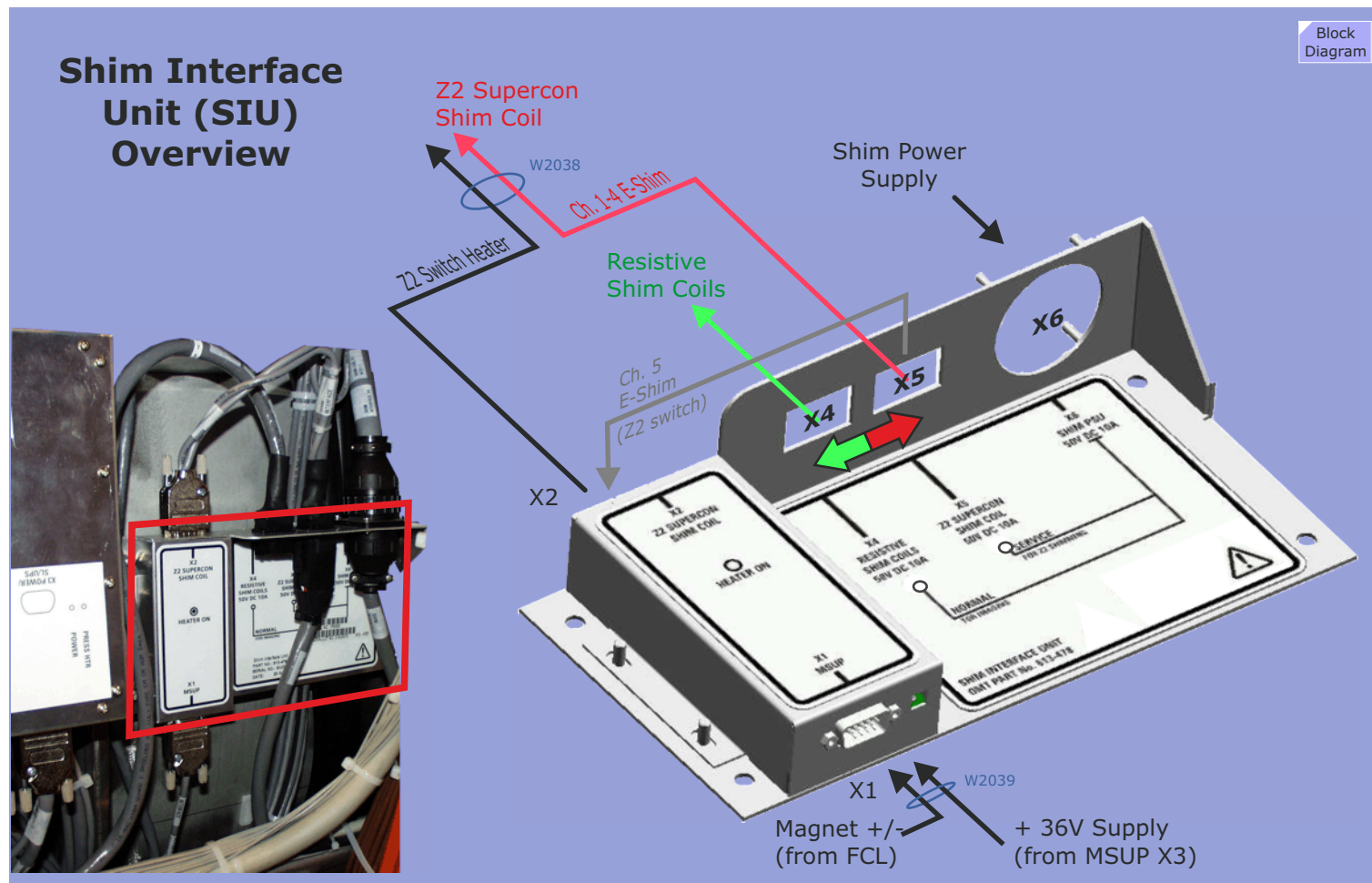
Figure 177 Shim Interface Unit Layout
