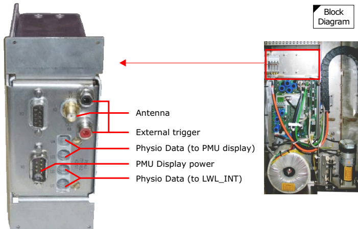
Figure 117 PDAU Layout
