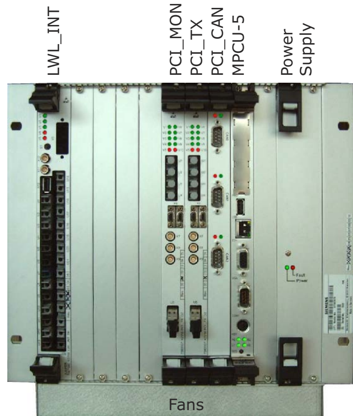
Figure 26 AMC Layout
