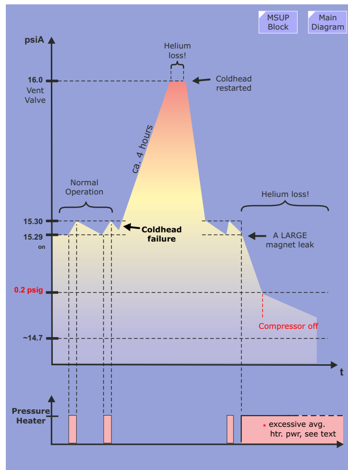
Figure 170 Magnet Pressure Regulation Scheme
