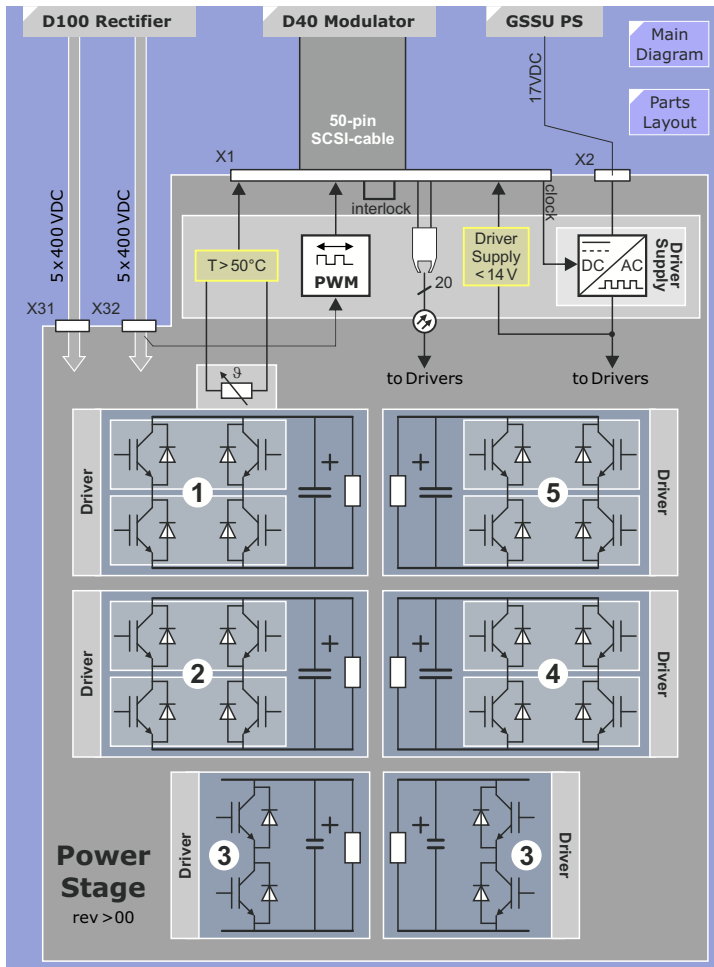
Figure 151 One Power Stage Module
