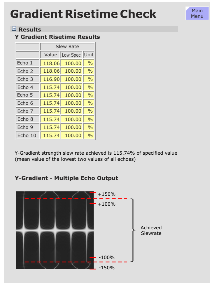
Figure 246 Gradient Risetime Check
